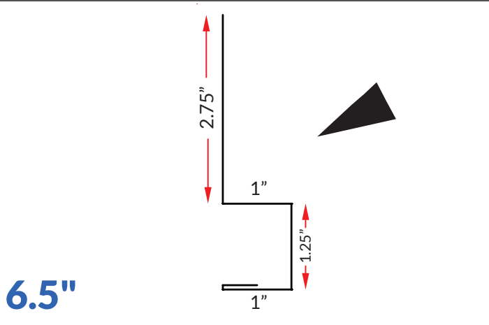
7/8 BOX BASE
