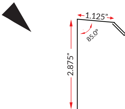
7/8 REVERSE DRIP
