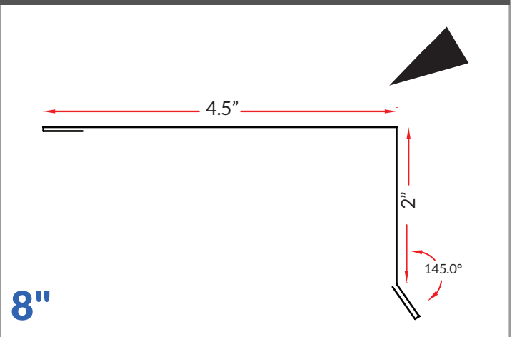
7/8 CORRUGATED GABLE
