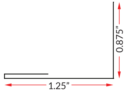
7/8 2PC J CHANNEL (2 OF 2)
