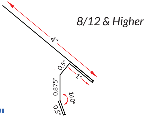
HI PITCH LOCKING EAVE
