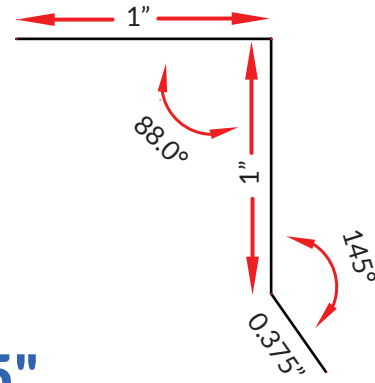
GABLE CLEAT
