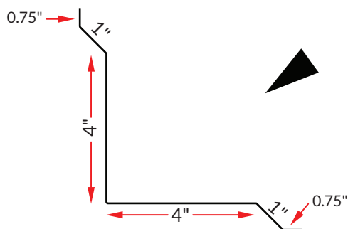
INSIDE CORNER
