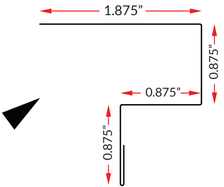
3/4" DOUBLE J
