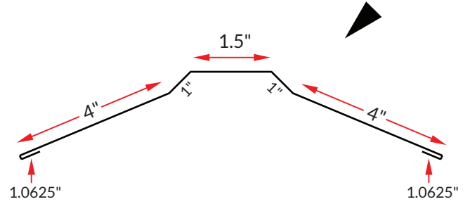
RIDGE CAP
