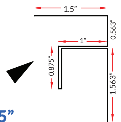
1/2"-3/4" INSIDE CORNER
