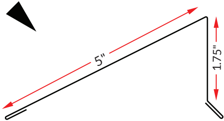
PEAK CAP
