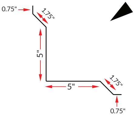
INSIDE CORNER
