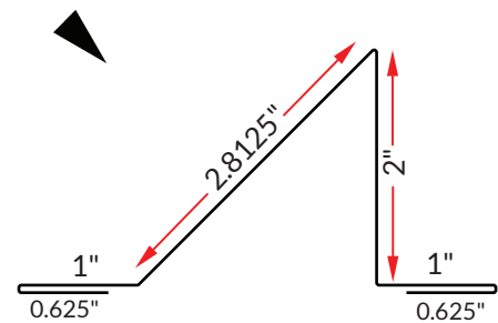
SNOW STOP
