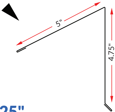
PEAK CAP
