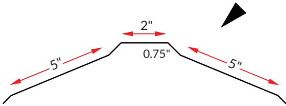
RIDGE CAP
