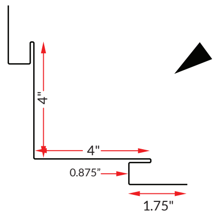
INSIDE CORNER
