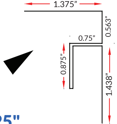
1/2"-1/2" INSIDE CORNER
